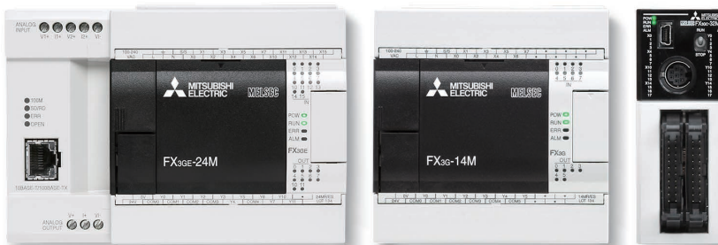
Standard Model
