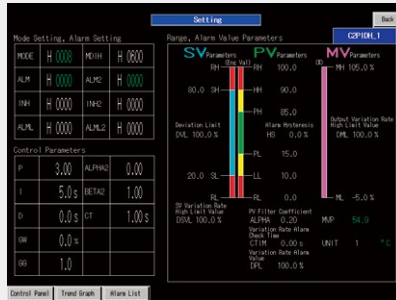
Tag setting screen
