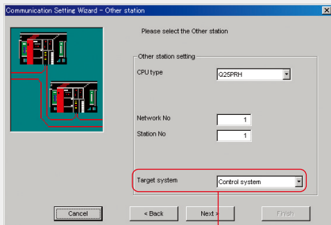
Select "Control system" for the redundant system.
