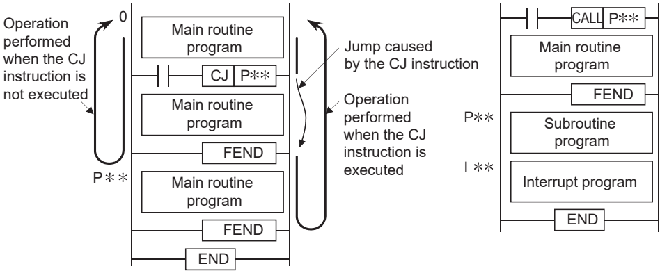
(a) When the CJ instruction is used (b) When there are subroutine and interrupt programs
