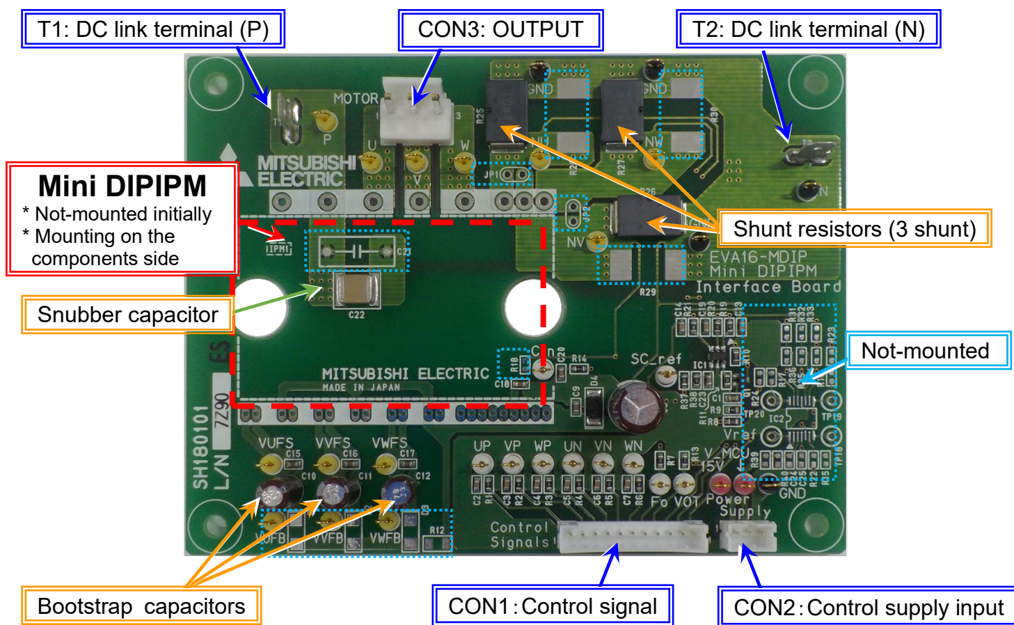
Fig.5-1-2 Demo board EVA16-MDIP photo
