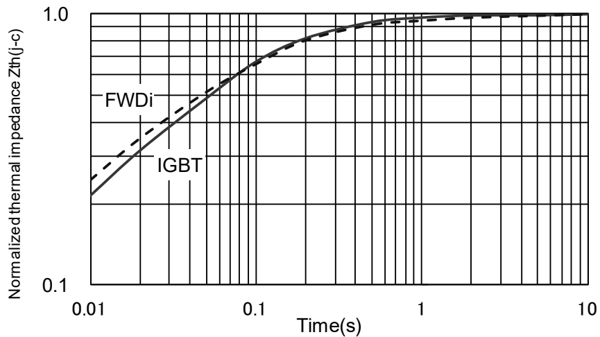
Fig.2-1-2 Typical transient thermal impedance (PSSxxS73F6)
