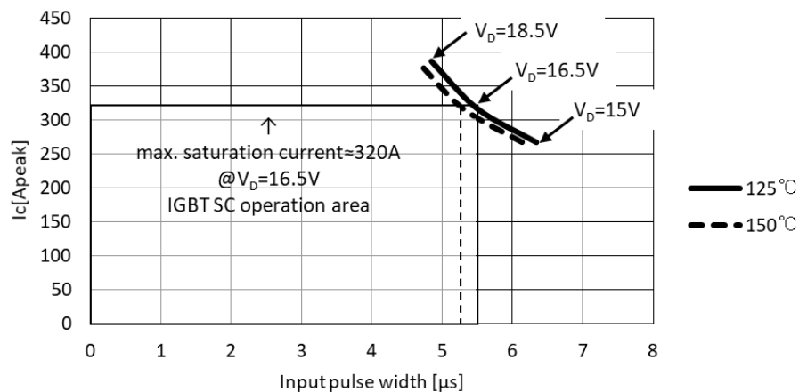
Fig.3-1-17 Typical SCSOA curve of PSS50S73F6
