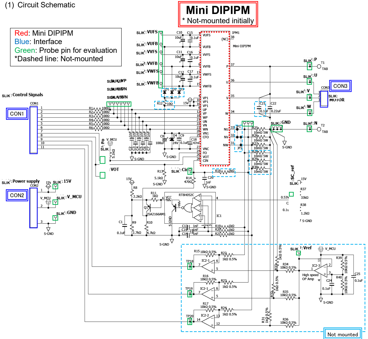
Fig.5-3-1 Demo board circuit schematic
