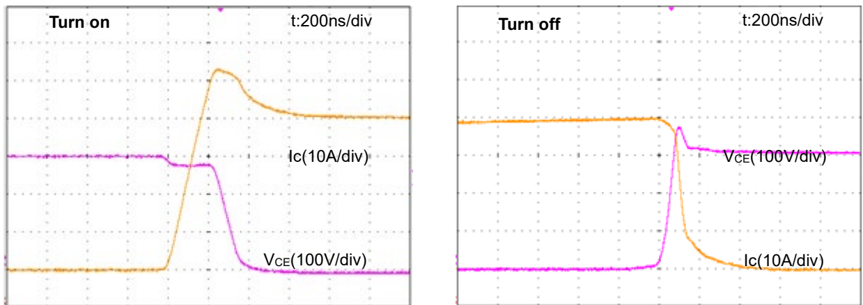
Fig.2-1-5 Typical switching waveform (PSS20S73F6) Conditions: V CC =300V, V D =V DB =15V, T j =125°C, I C =20A, Inductive load half-bridge circuit
