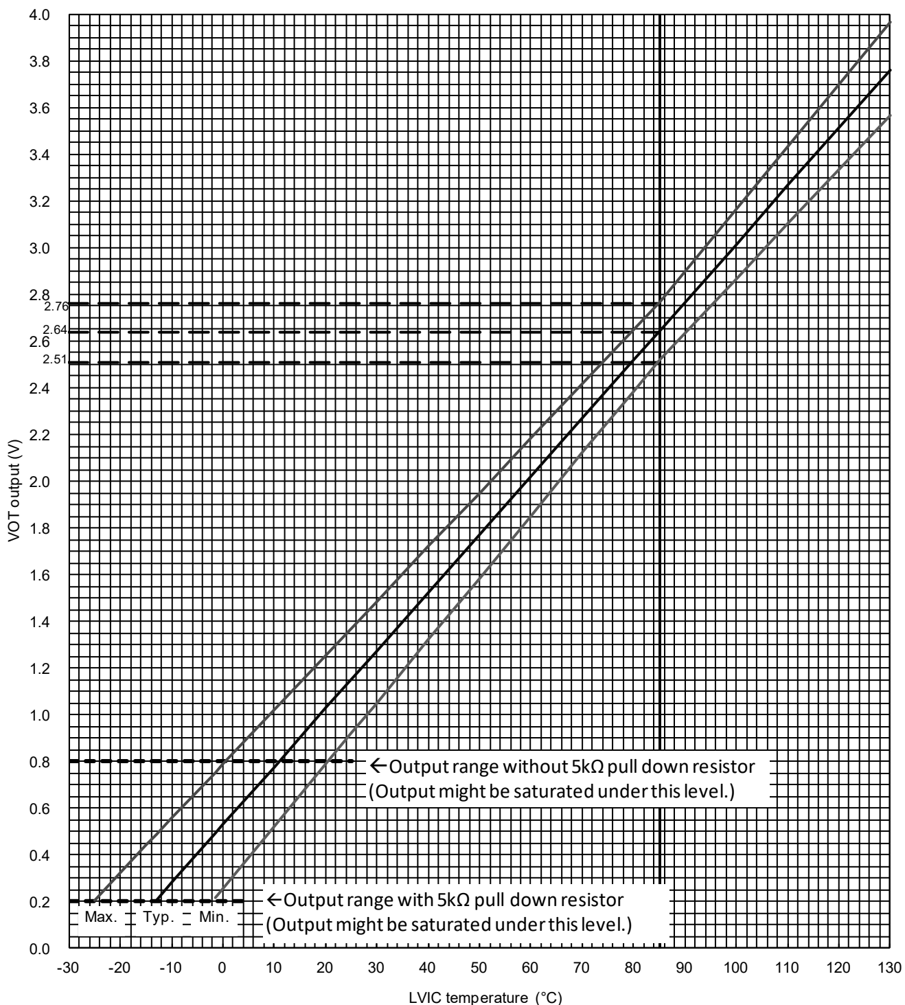
Fig.2-2-12 V OT output vs. LVIC temperature (PSSxxS73F6)
