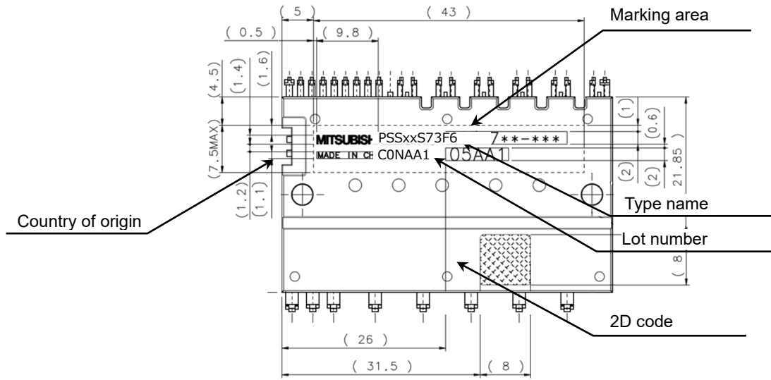
Fig.2-3-4 Laser marking view PSSxxS73F6 (Dimension in mm)
