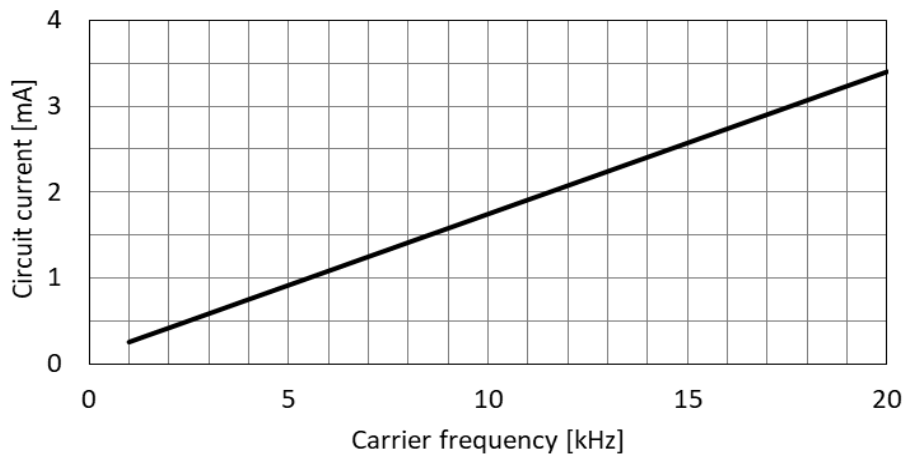
Fig.4-2-2 I_{DB} vs. Carrier frequency for PSS30S73F6
