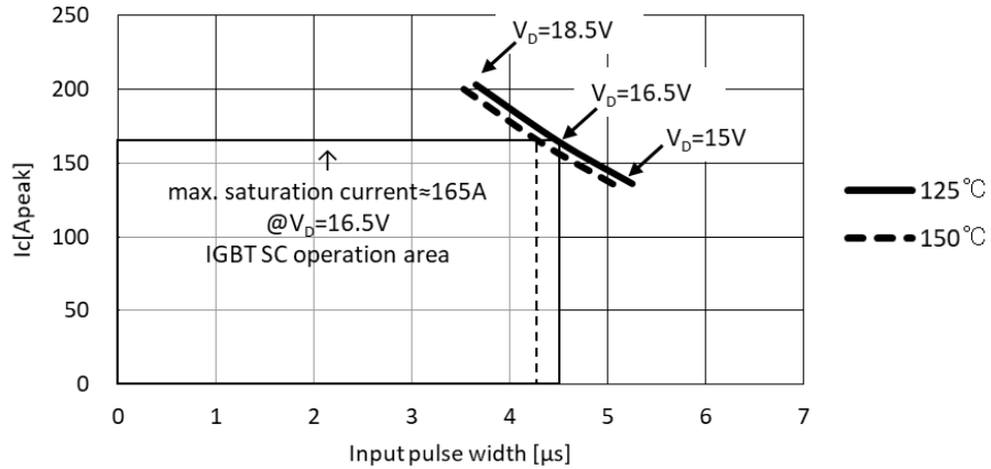
Fig.3-1-15 Typical SCSOA curve of PSS20S73F6
