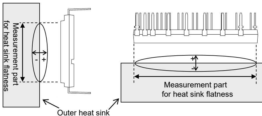
Fig.2-4-3 Measurement point of heat sink flatness (PSSxxS73F6)
