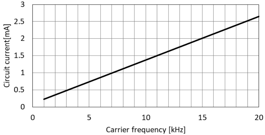
Fig.4-2-1 I_{DB} vs. Carrier frequency for PSS20S73F6
