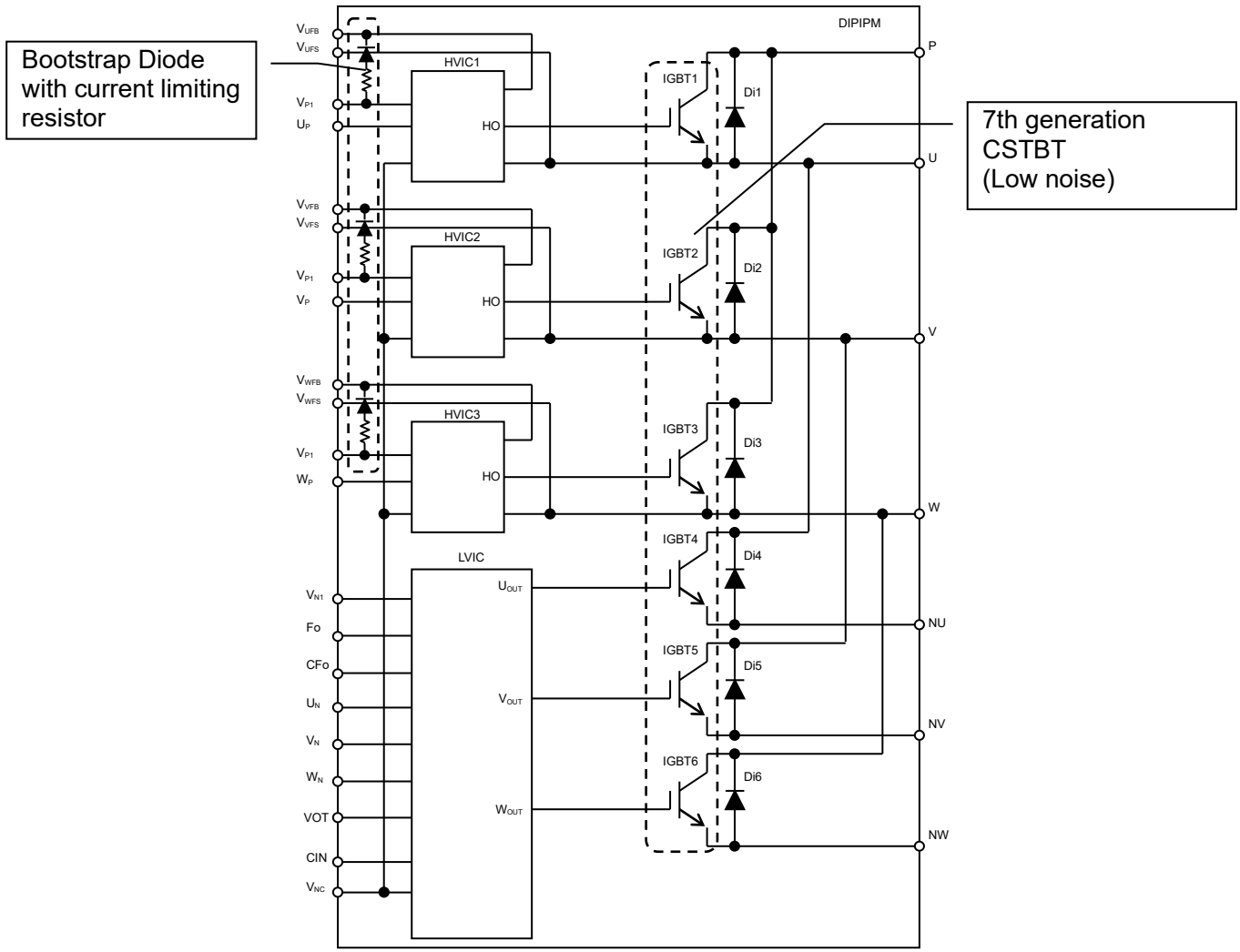
Fig.1-2-1 Inner block diagram
