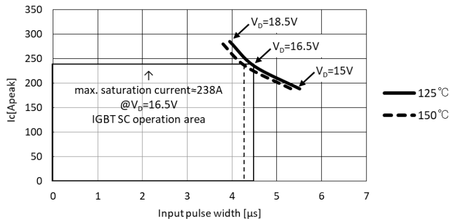
Fig.3-1-16 Typical SCSOA curve of PSS30S73F6
