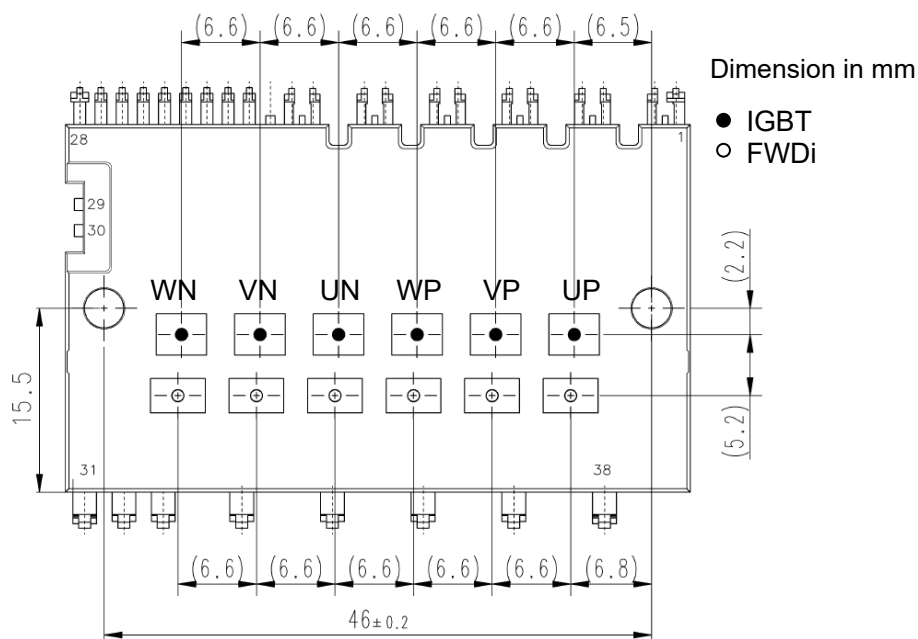
Fig.2-1-1 Power chip position (PSSxxS73F6)
