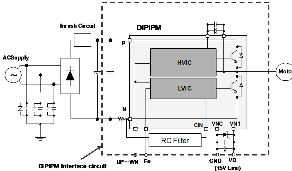
Fig.5-1-1 Demo board interface circuit (EVA16-MDIP)
