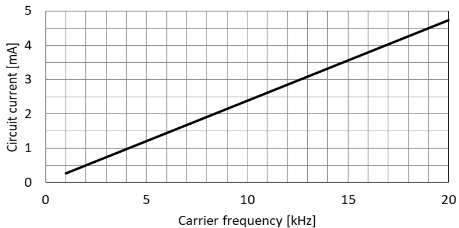
Fig.4-2-3 I_{DB} vs. Carrier frequency for PSS50S73F6
