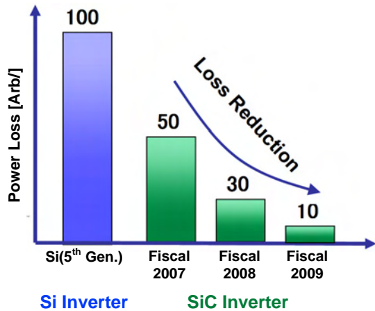
Fig. 6 Progress in power loss reduction of SiC inverter by MELCO
