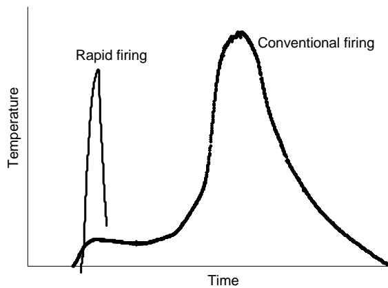
Fig. 5 Comparison of firing profiles
