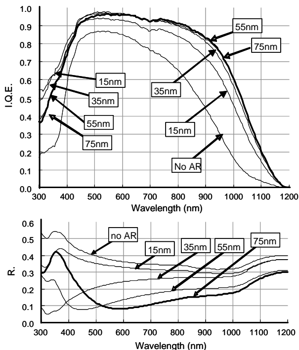
Fig. 3 Dependence of IQE and reflectivity on AR coating thickness
