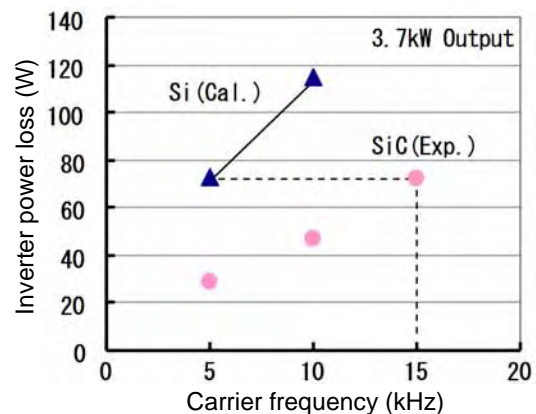
Fig. 2 Dependency of inverter power loss on PWM carrier frequency at 3.7 kW output
