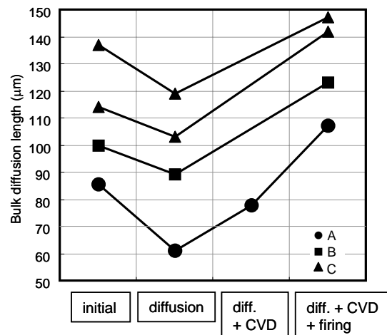
Fig. 2 Change in diffusion length with process steps (A, B, C: suppliers)
