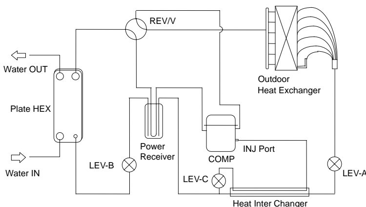
Fig. 4 Refrigerant circuit
