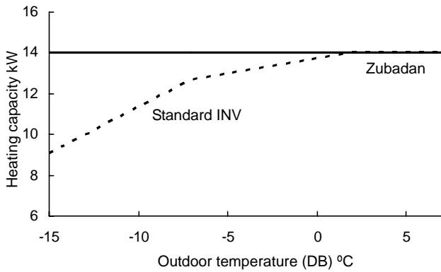
Fig. 6 Heating capacity characteristics of Zubadan
