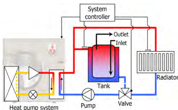
Fig. 1 Typical ATW system in Europe
