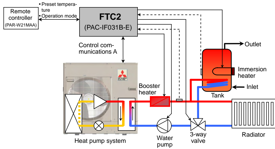
Fig. 9 ATW system with FTC2
