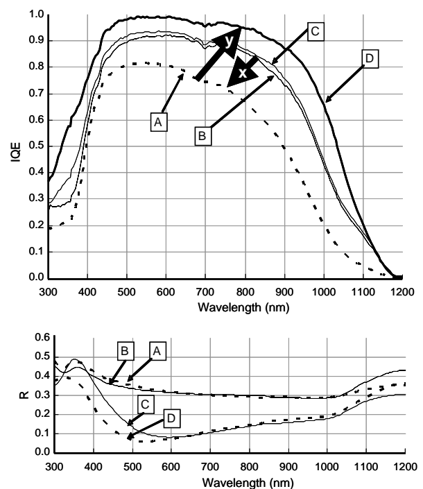
Fig. 4 Effect of metallization process on diffusion length
