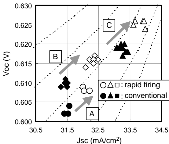
Fig. 6 Enhancement of V_{oc} and J_{sc} by rapid firing
