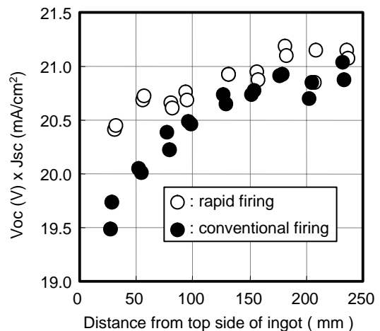
Fig. 7 Enhancement V_{oc} \times J_{sc} (life time) by rapid firing
