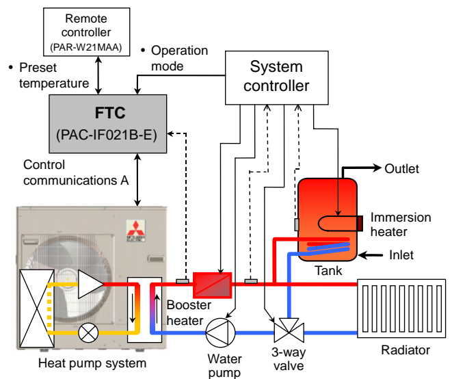
Fig. 8 ATW system with FTC
