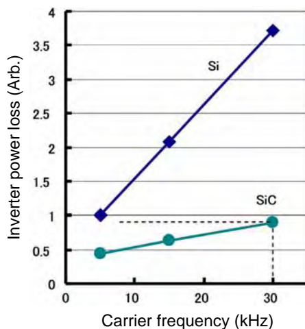
Fig. 4 Dependency of inverter power loss on PWM carrier frequency at 11 kW output
