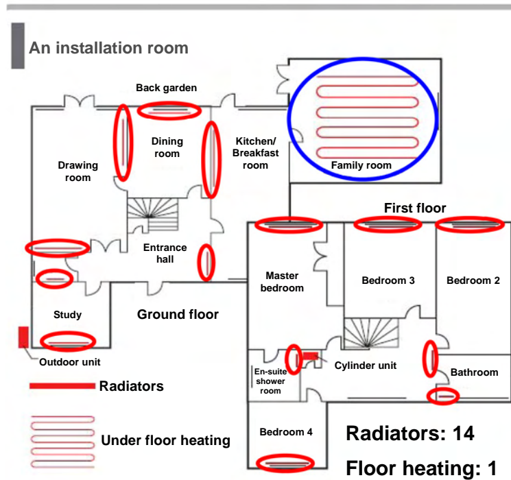
Fig. 3 House layout for demonstration test
