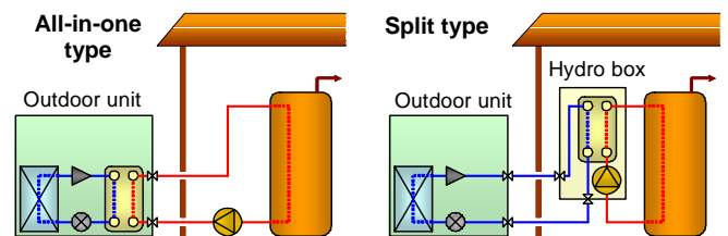
Fig. 2 Types of ATW outdoor unit
