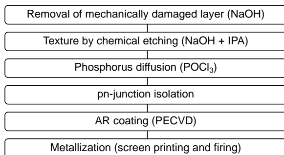
Fig. 1 Fundamental process sequence for the cells
