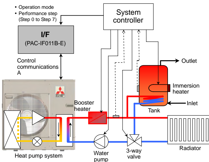
Fig. 7 ATW system with I/F
