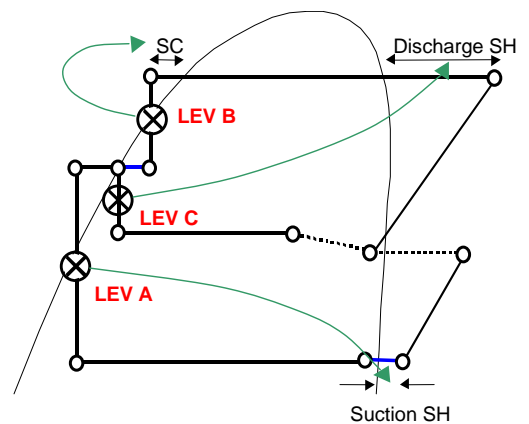
Fig. 5 LEV control during injection operation
