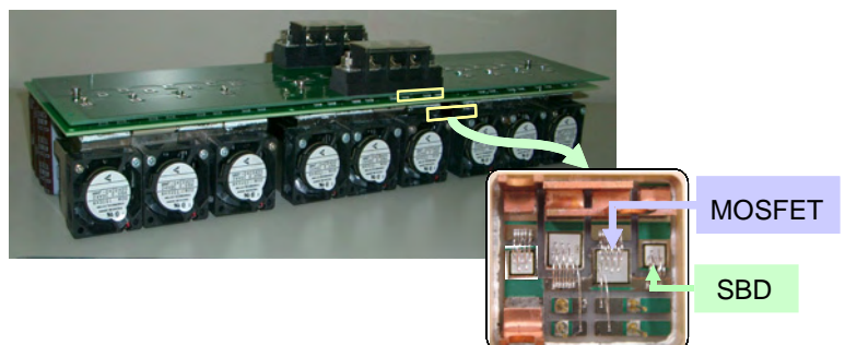
Fig. 5 Ultra-low loss 400-V/22-kW class SiC inverter and SiC module
