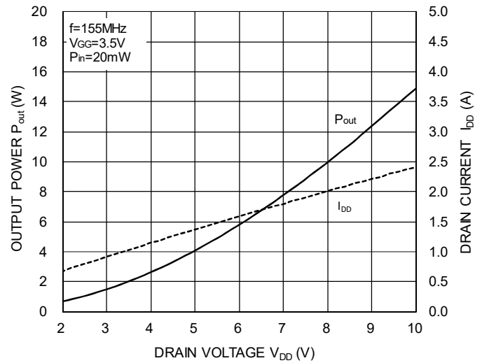
OUTPUT POWER, DRAIN CURRENT versus DRAIN VOLTAGE
