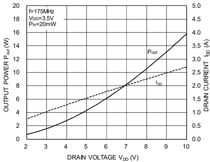
OUTPUT POWER, DRAIN CURRENT versus DRAIN VOLTAGE
