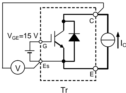
V_{CEsat} characteristics test circuit
