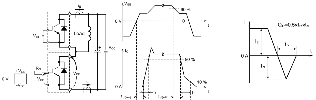
Switching test circuit and waveforms
