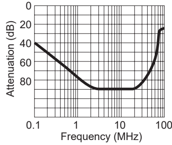
Fig.3. Damping characteristics of noise filter
