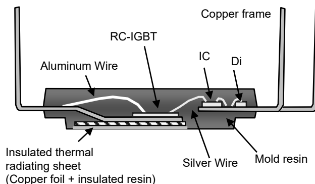
Fig.1-1-2 Internal cross-section structure
