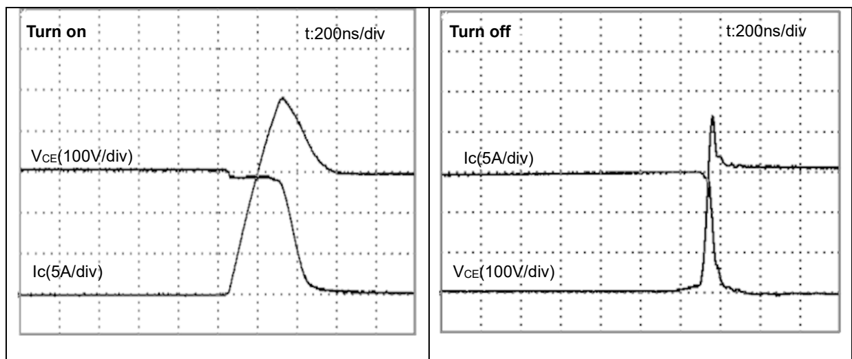
Fig.2-1-7 Typical switching waveform (SLIMDIP-L) Conditions: V_{CC}=300\text{V} , V_D=V_{DB}=15\text{V} , T_j=125^\circ\text{C} , I_C=15\text{A} , Inductive load half-bridge circuit
