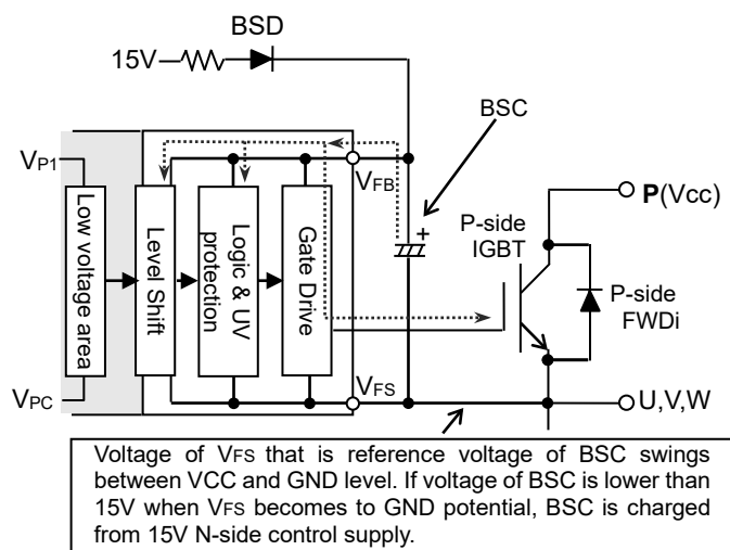
Fig.4-1-2 Bootstrap Circuit Diagram
