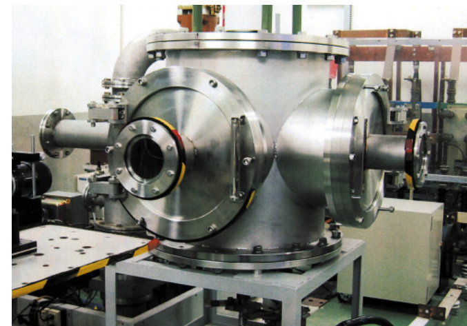
Demountable chamber
