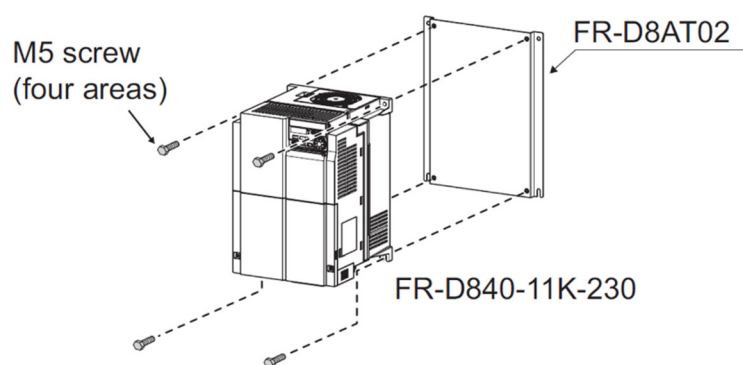
Installation example
