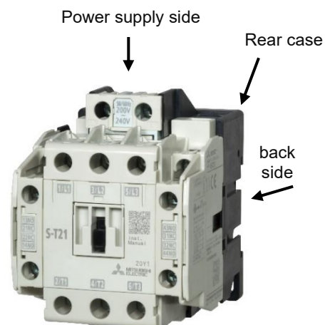
Fig1: Product Appearance (S-T21)
