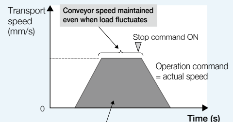
Good repeated operating pattern precision * Consistent operation pattern area can be ensured with fixed-position conveyance
