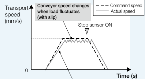
Variation in repeated operating pattern precision * Without sensorless servo control
