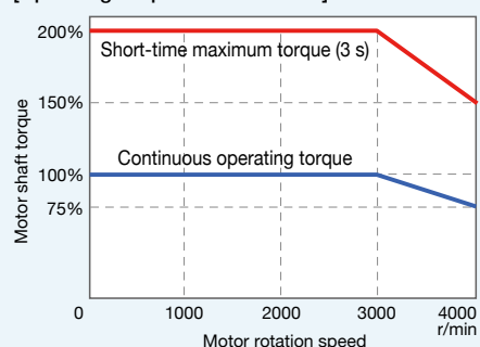
[Operating torque characteristics]
