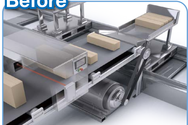
[Current] Mitsubishi inverter + General purpose motor (+ proximity sensor)
