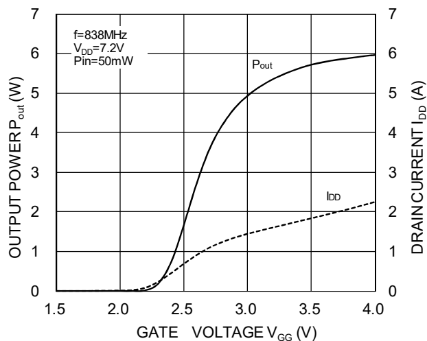
OUTPUT POWER and DRAIN CURRENT versus GATE VOLTAGE
