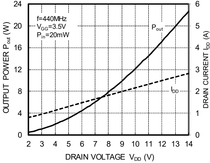
OUTPUT POWER and DRAIN CURRENT versus DRAIN VOLTAGE
