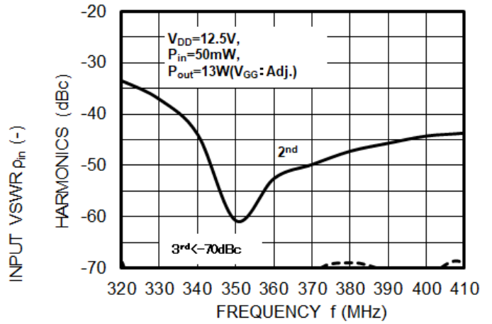
2 nd , 3 rd HARMONICS versus FREQUENCY
