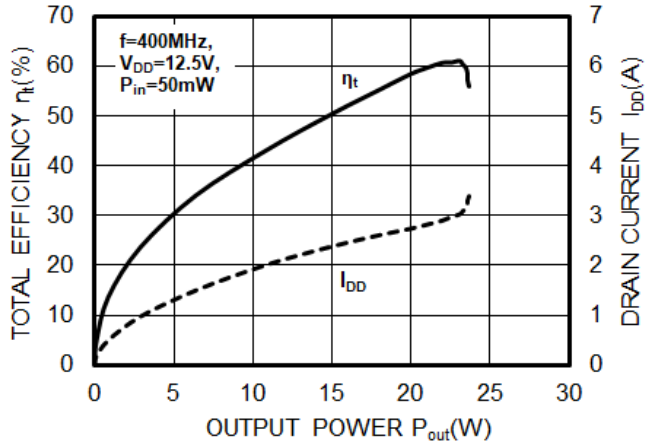
TOTAL EFFICIENCY and DRAIN CURRENT versus OUTPUT POWER
