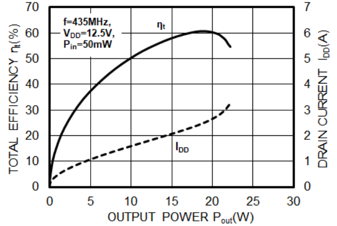
TOTAL EFFICIENCY and DRAIN CURRENT versus OUTPUT POWER
