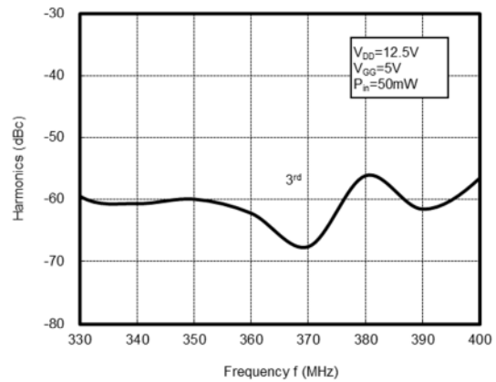
3 rd HARMONICS versus FREQUENCY
