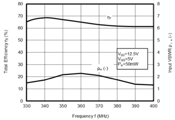
TOTAL EFFICIENCY, INPUT VSWR versus FREQUENCY
