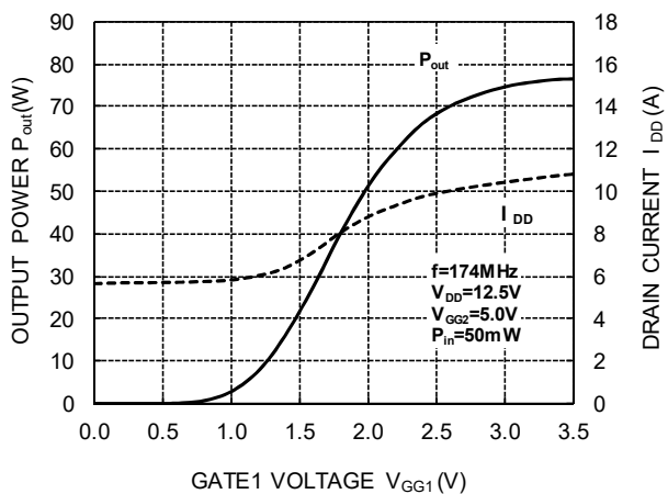
OUTPUT POWER and DRAIN CURRENT versus GATE VOLTAGE1
