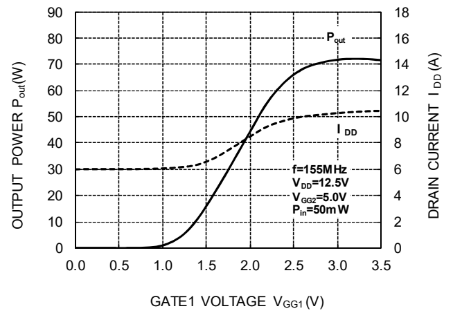
OUTPUT POWER and DRAIN CURRENT versus GATE VOLTAGE1
