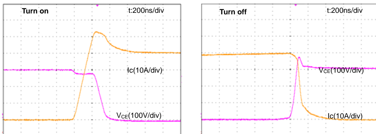
Fig.2-1-5 Typical switching waveform (PSS20S73F6)
