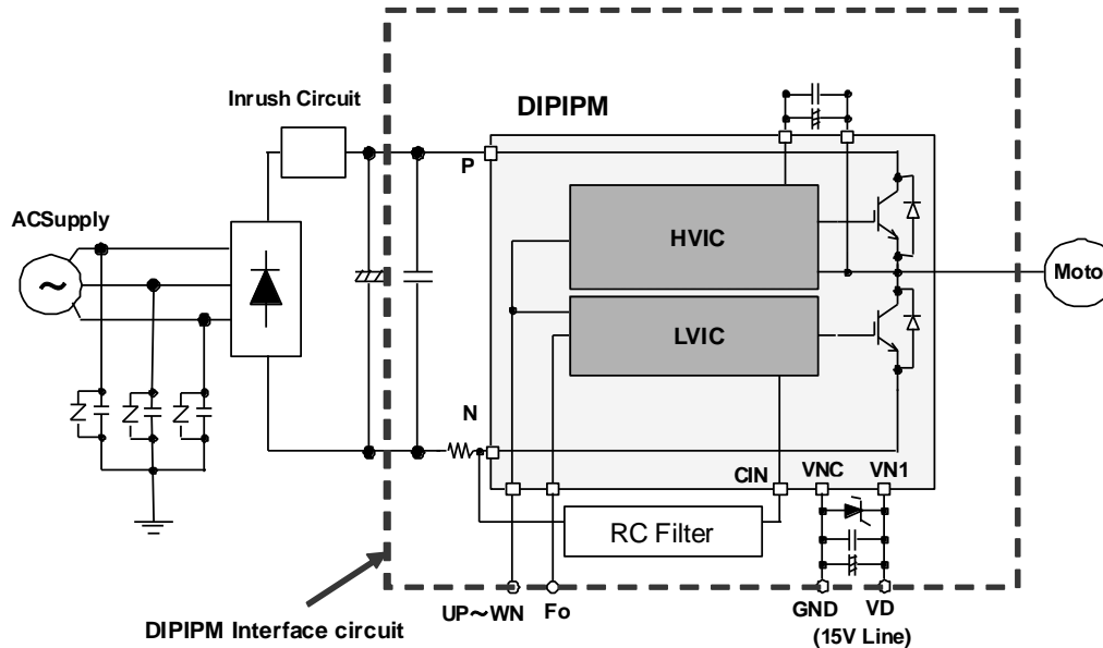
Fig.5-1-1 Demo board interface circuit (EVA16-MDIP)
