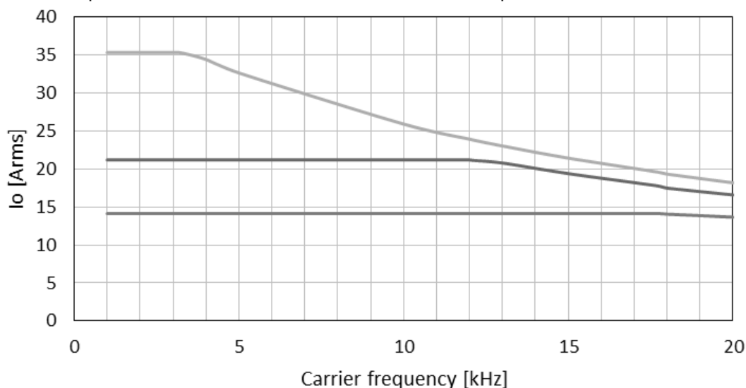
Fig.3-2-2 Effective current-carrier frequency characteristics
