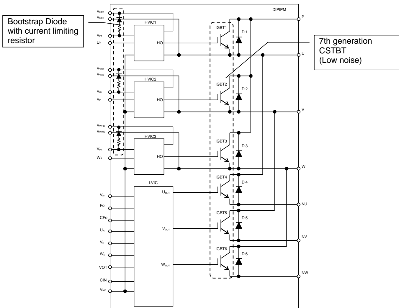
Fig.1-2-1 Inner block diagram
