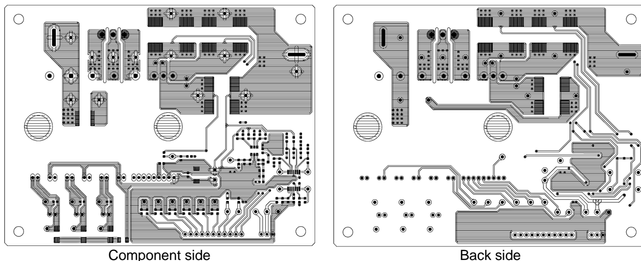
Fig.5-2-1 Demo board component layout (DIIPM is mounted to back side.)
