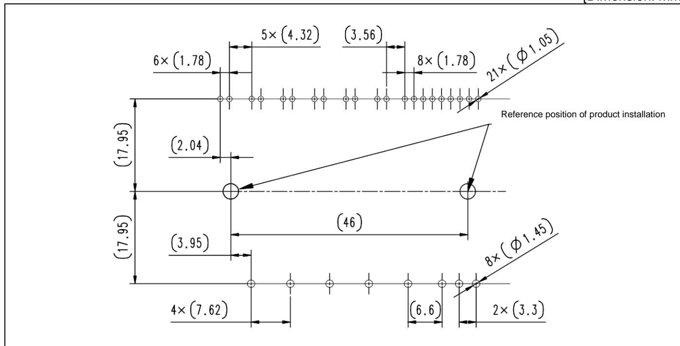
Fig.2-3-2 PCB through-hole pattern of PSSxxS73F6 (Reference Figure)
