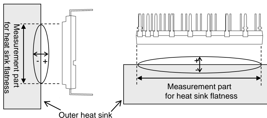
Fig.2-4-2 Measurement point of heat sink flatness
