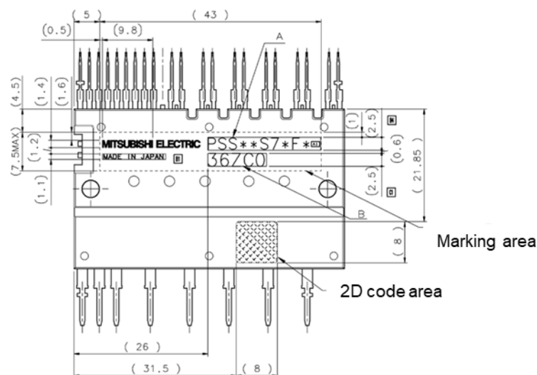
Fig.2-3-3 Laser marking view PSSxxS73F6 (Dimension in mm)
