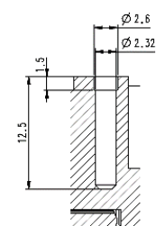
SECTION B
