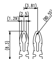
SECTION B
