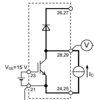
Brake IGBT
