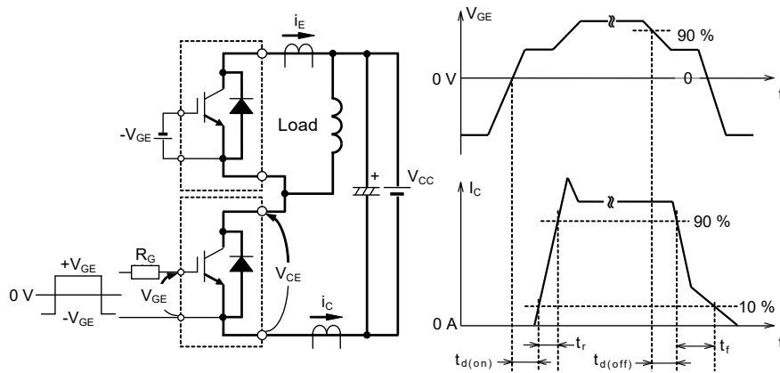
Switching test circuit and waveforms
