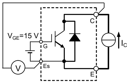
V_{CEsat} characteristics test circuit
