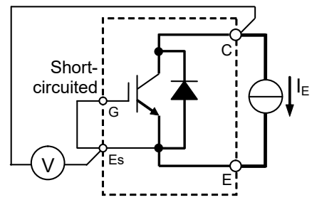
V_{EC} characteristics test circuit
